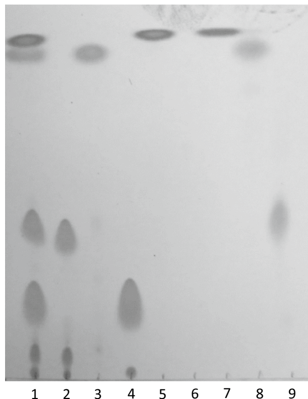
Figure 6. Thin layer chromatogram of human skin swab extract fractionated on a normal phase silica gel plate. Lane assignments are as follows: 1—All standards (trilinolein [20 \mu\text{g} ], jojoba oil [20 \mu\text{g} ], linoleic acid [20 \mu\text{g} ], squalene [10 \mu\text{g} ]), 2—trilinolein (20 \mu\text{g} ), 3—jojoba oil (20 \mu\text{g} ), 4—linoleic acid (20 \mu\text{g} ), 5—squalene (10 \mu\text{g} ), 6—blank, 7—hexane fraction (0.1 BE), 8—2% ether (in hexane) fraction (0.1 BE), 9—5% ether (in hexane) fraction (0.1 BE).
